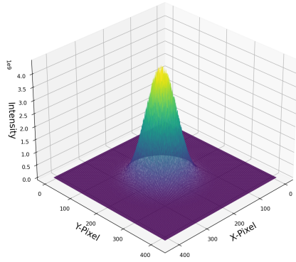
Figure 9: To the left is a 3D intensity plot of the pink beam, to the right the 3D intensity plot of the monochromatic beam with the same attenuators in.
