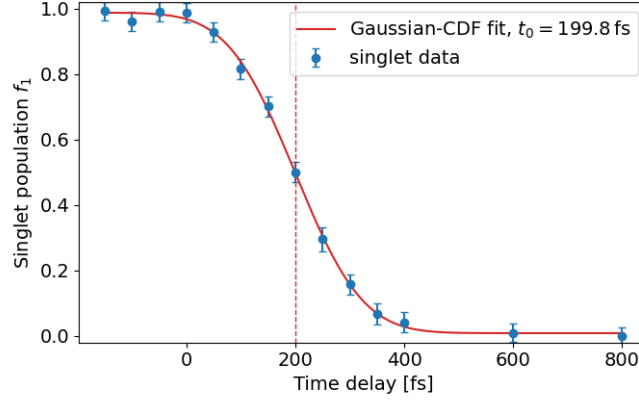
Figure 21: The fitted evolution of the singlet population.
